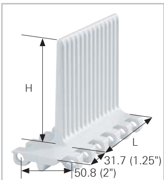
M506RFxx indent flight
